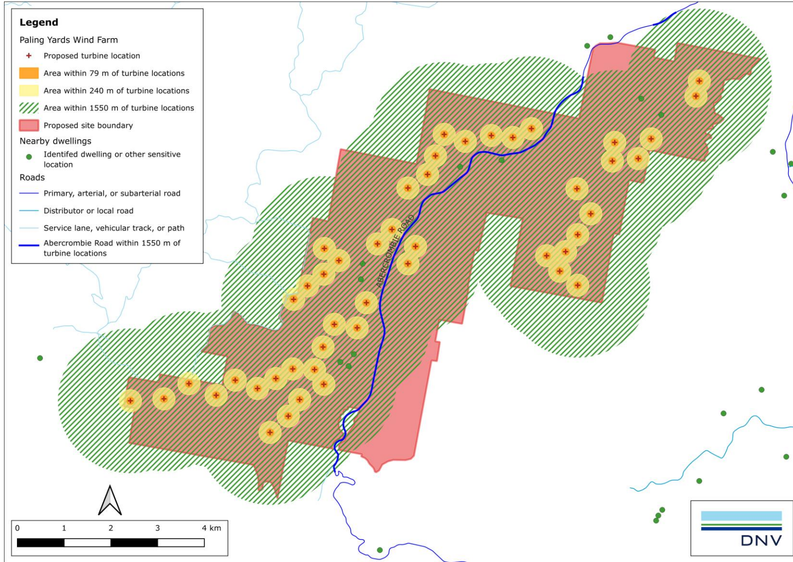
Figure 1 Locations of nearby dwellings and other sensitive locations, properties, and roads in relation to the proposed Project
